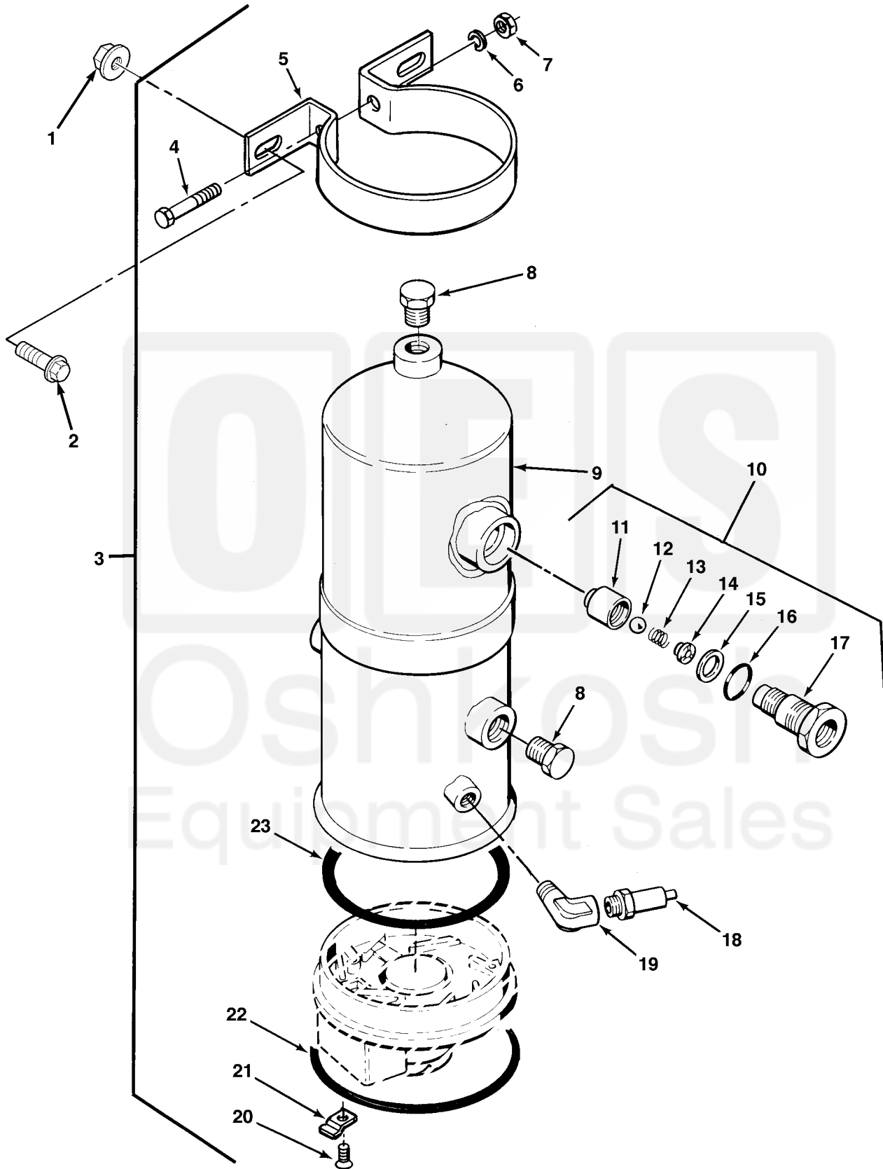
FIG.202 AIR DRYER
